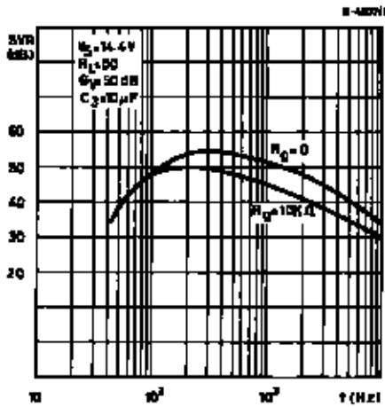
Figure 11 : Supply Voltage Rejection vs. Frequency.
