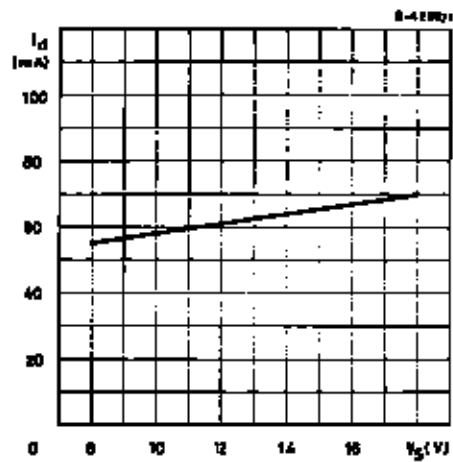
Figure 4 : Quiescent Drain Current vs. Supply Voltage.
